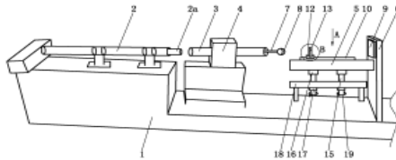
Figure 10.3 Part of the instruction manual on Wang Lijun's patented invention: "a collision machine to cause primary brain-stem injuries" 391
